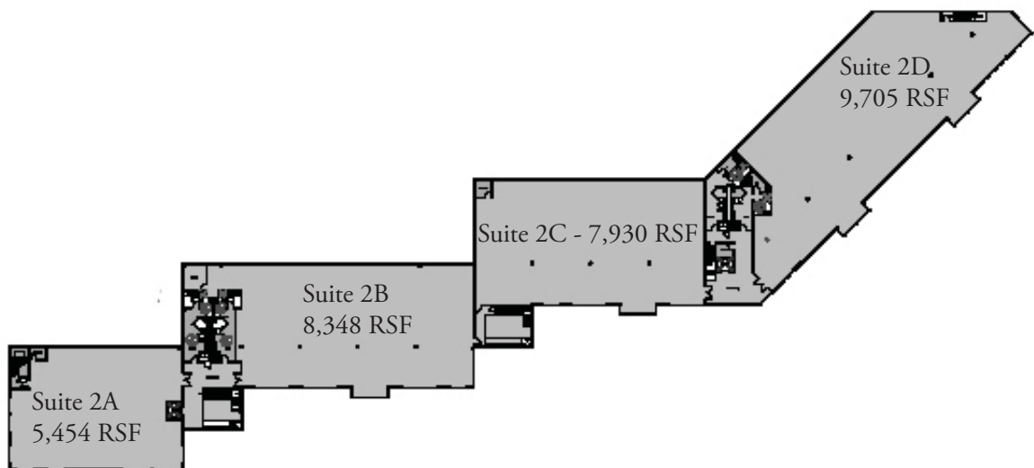
SECOND FLOOR
